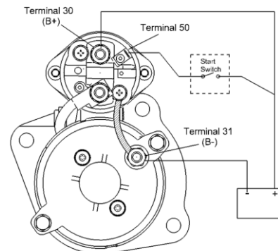
INSULATED RETURN
