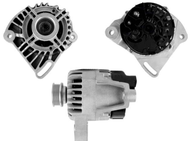
LEA1252 14V / 70A Replacing: 102211-8280
